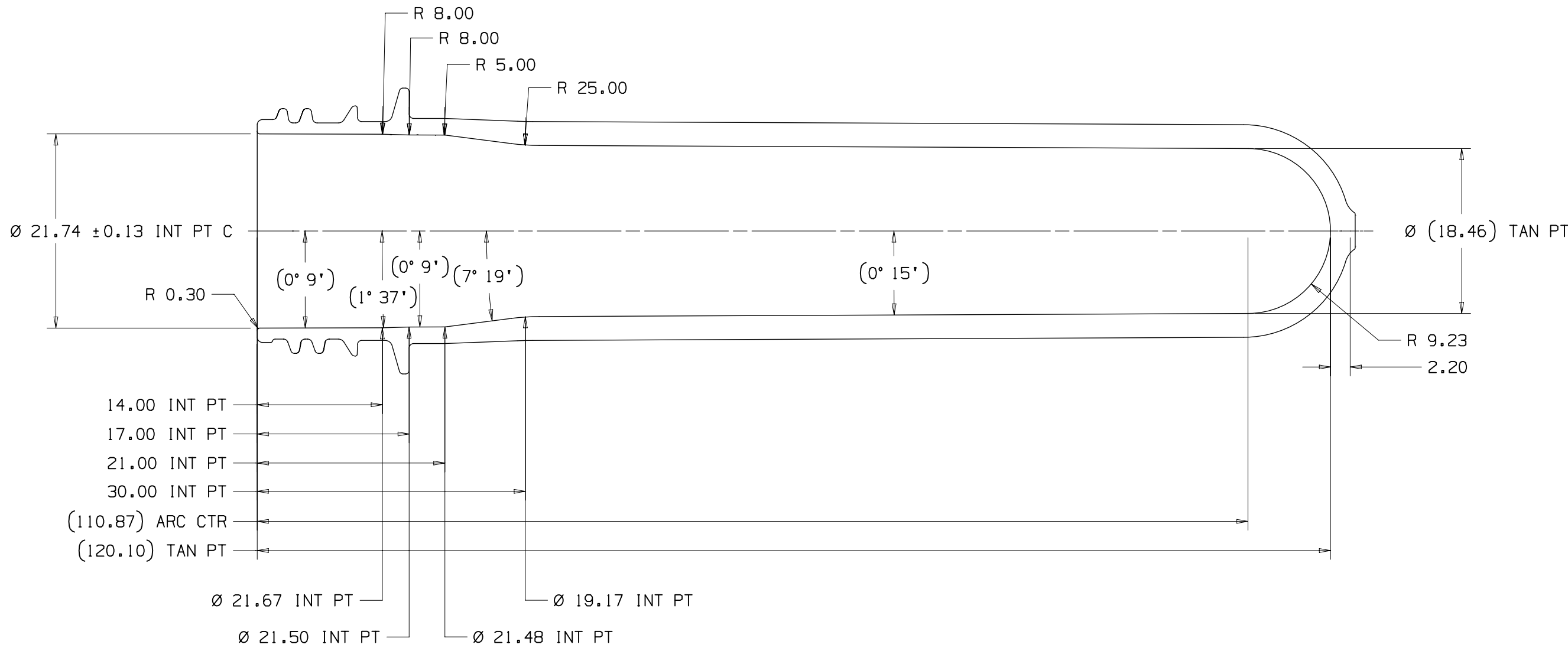
SECTION A-A CORE SIDE DIMENSIONS SCALE 2:1
