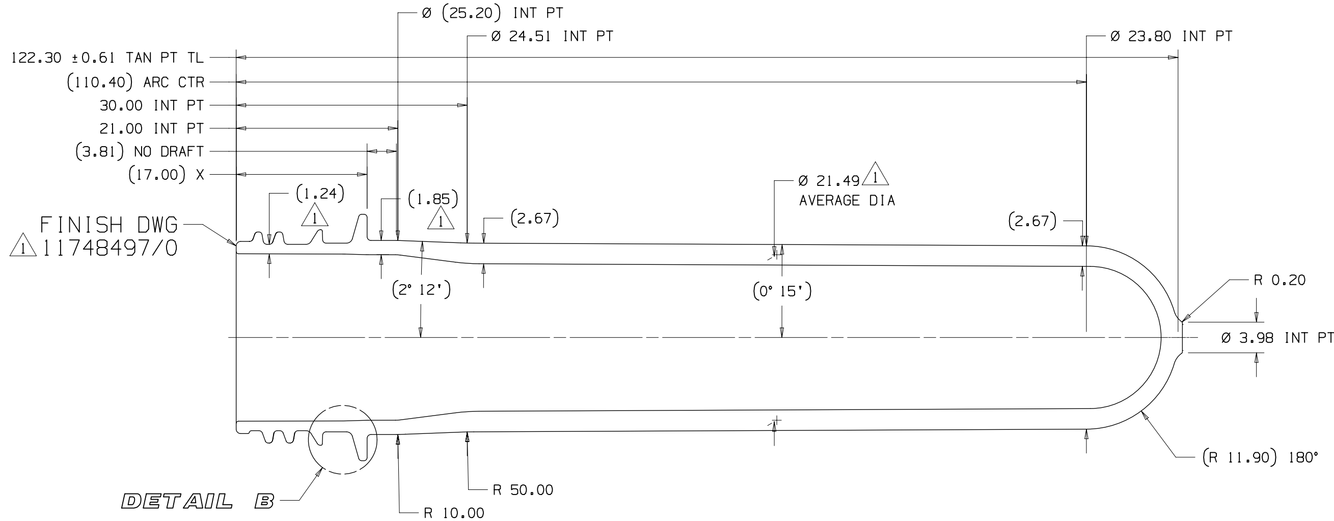
SECTION A-A CAVITY SIDE DIMENSIONS SCALE 2:1
