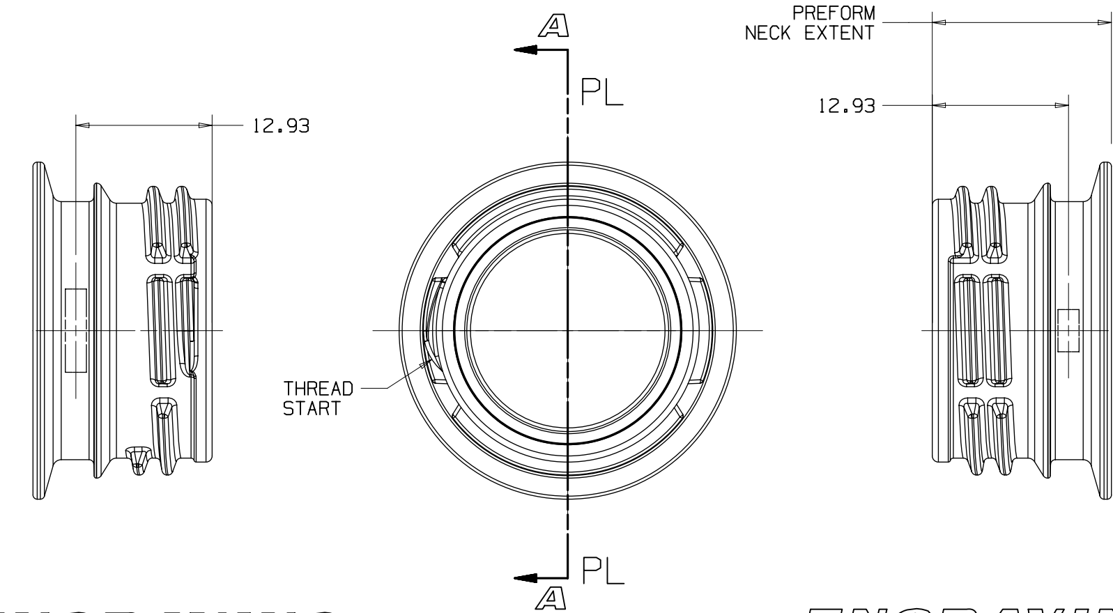
ENGRAVING VIEW SIDE A (OPERATOR) SCALE 2:1
