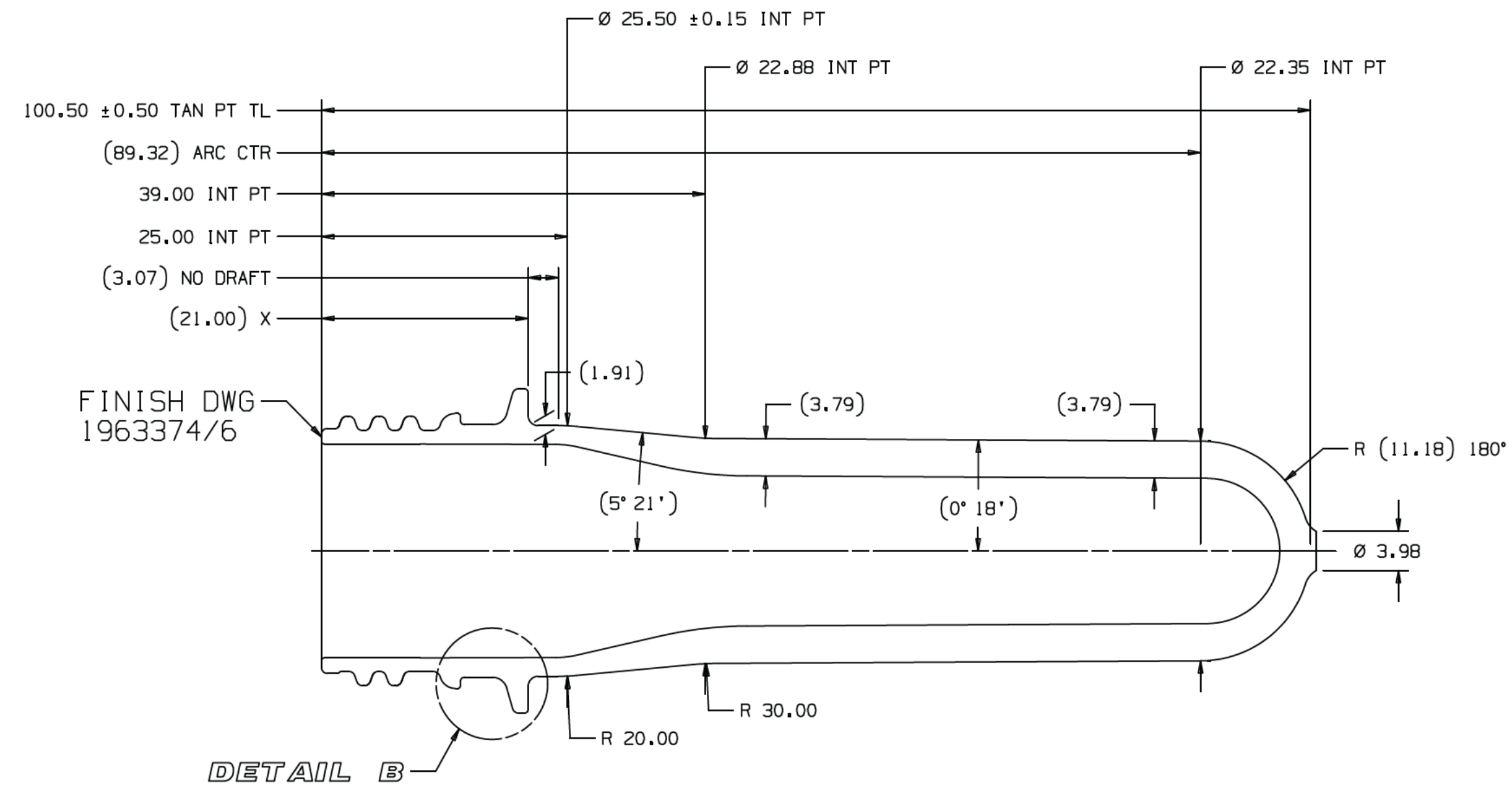
SECTION A-A CAVITY SIDE DIMENSIONS SCALE 2:1
