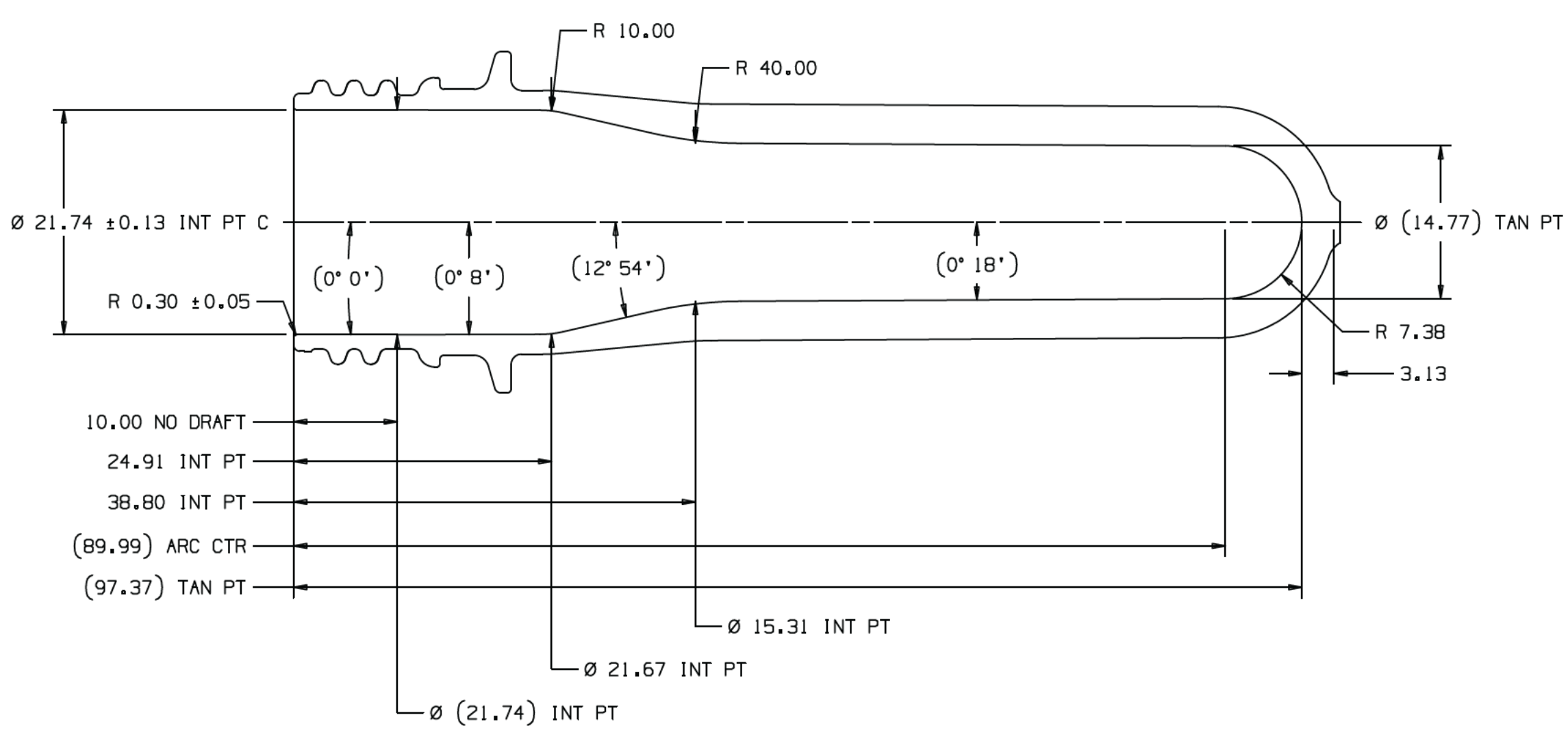
SECTION A-A CORE SIDE DIMENSIONS SCALE 2:1
