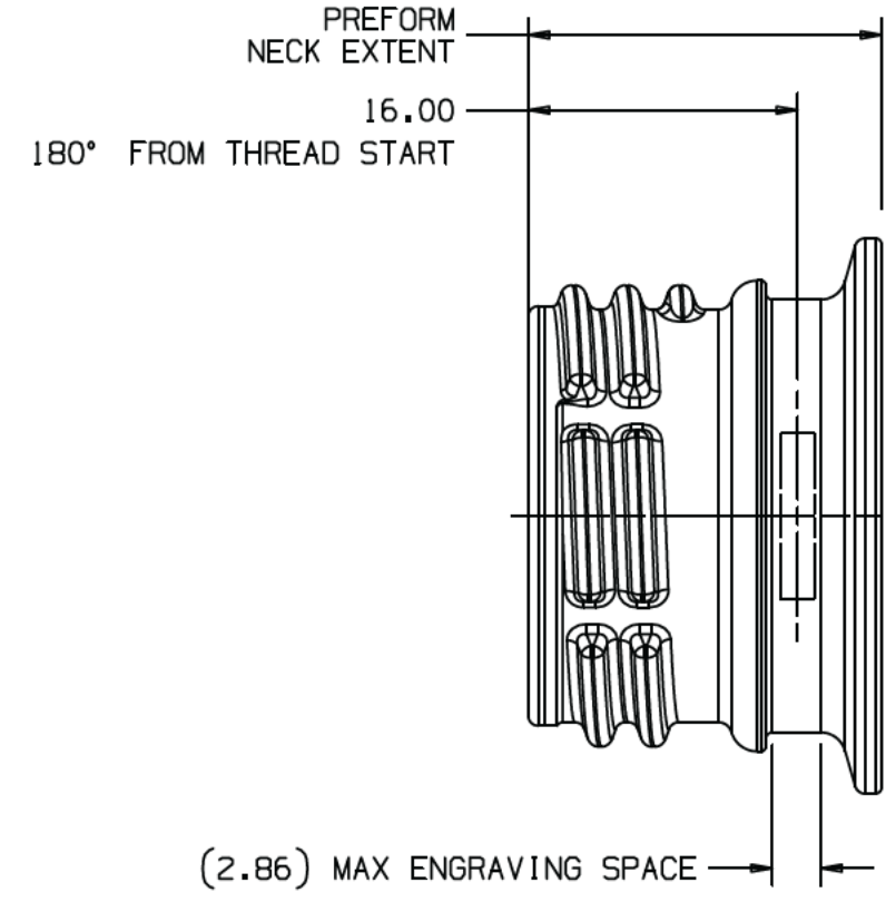
ENGRAVING VIEW SCALE 2:1
