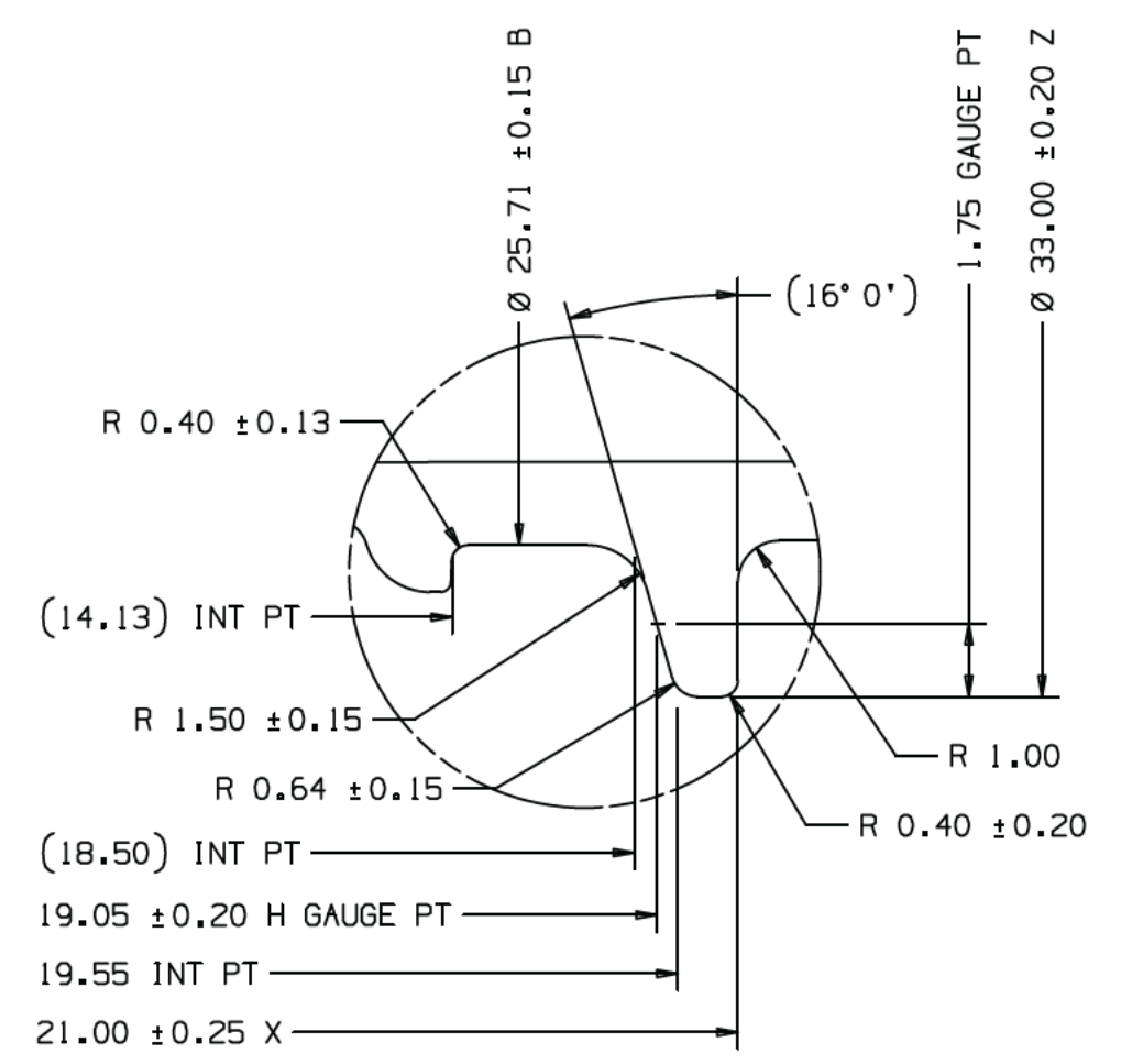
DETAIL B SCALE 5:1
